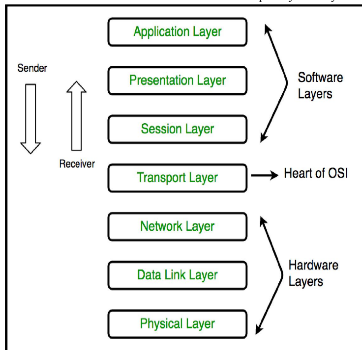
OSI MODEL
