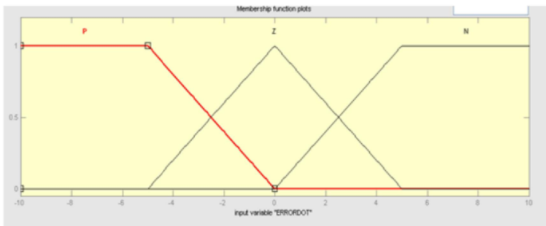
Figure 4: Error-Dot membership functions
