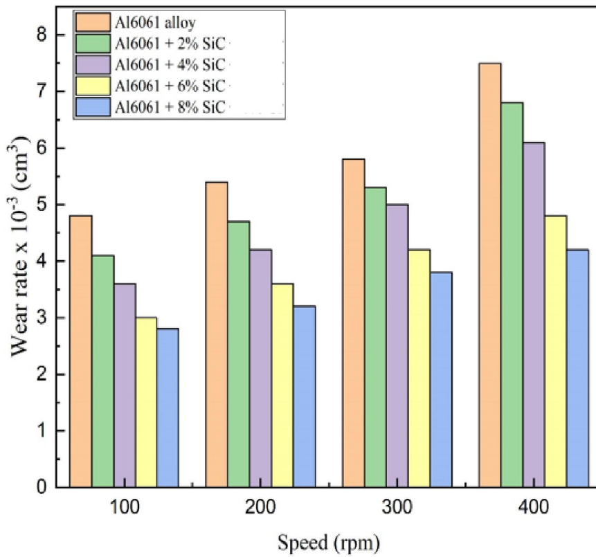
Figure 3: The wear rate composites at various sliding speeds
