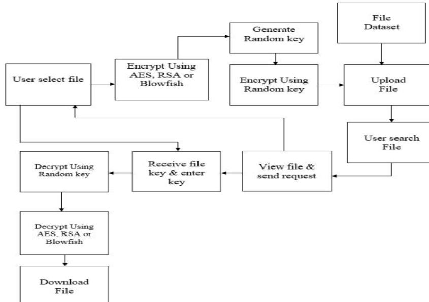
Fig 1. System Architecture
