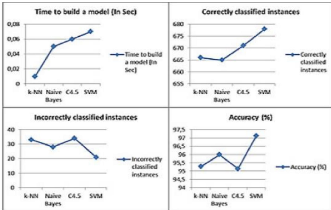
Fig. 1. Comparative graph of different classifiers.
