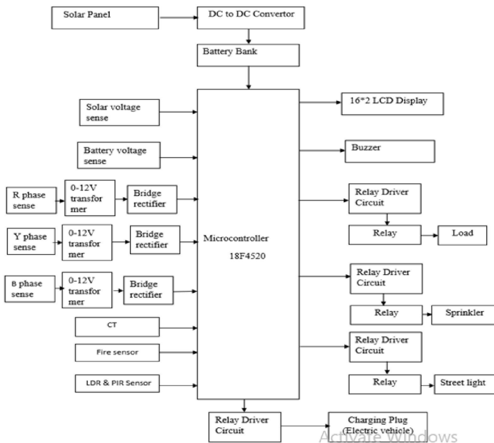
Figure 1: Block Diagram
