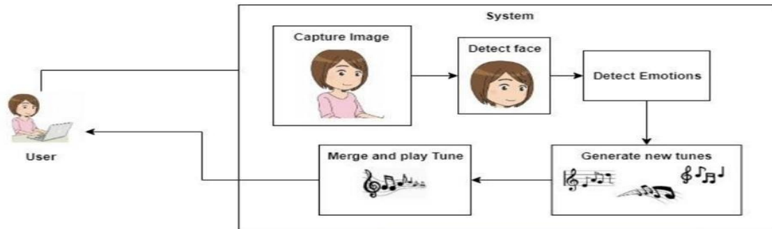
Figure 4.4: Class Diagram
