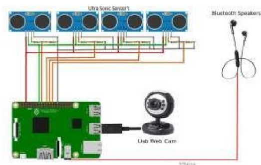
Fig 2.- Architecture Diagram
