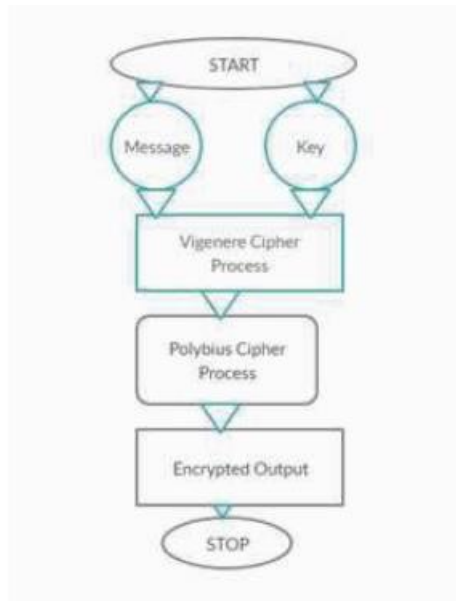
Flow chart of Hybrid algorithm.
