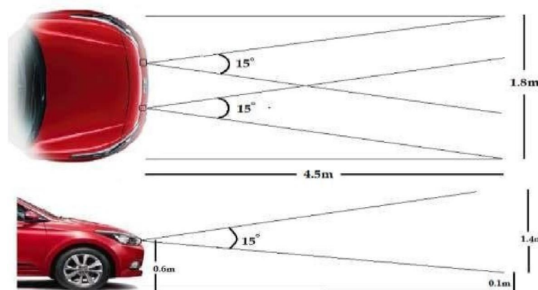
Figure 4.8 Ultrasonic sensor position
