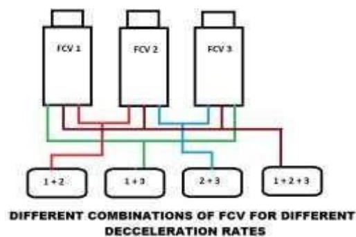
.Figure 4.1 Braking fluid distributions DOI: 10.48175/568
