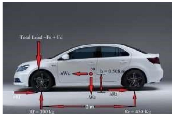
Figure 2.11 Force distribution
