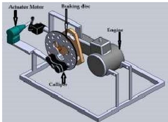
Figure 4.2 Schematic setup
