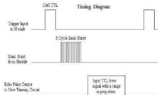
Figure 2.4 Timing diagram of Ultrasonic sensor
