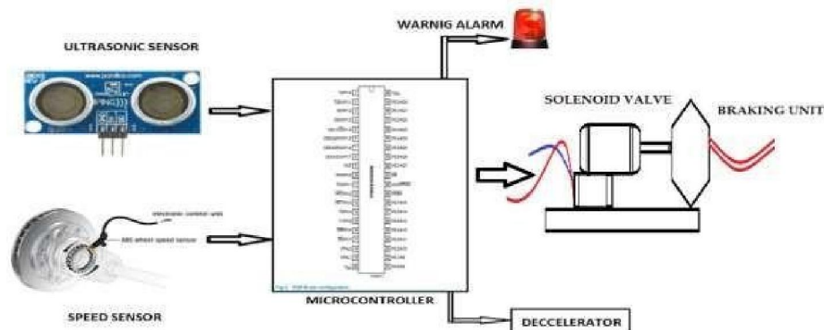
Figure 2.2 System layout
