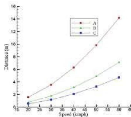
Figure 4.7 Graph of Speed Vs Stopping distance
