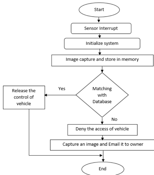
Fig- 6: Flowchart
