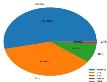
Pie chart distribution of multi-class labels
