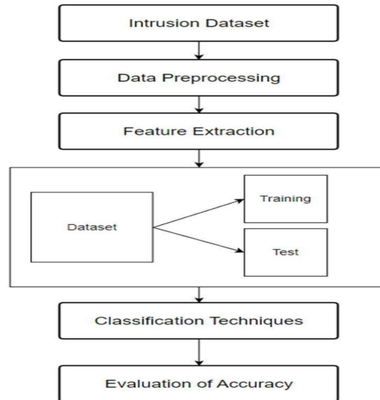
Fig 5.1 System Architecture
