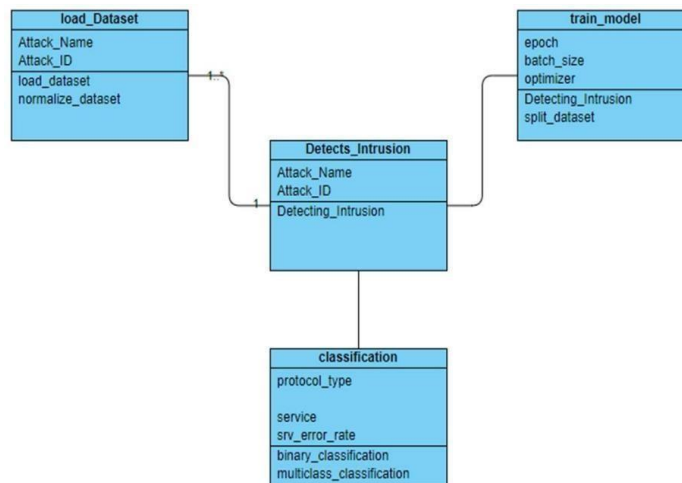
Fig 4.2 Class Labels
