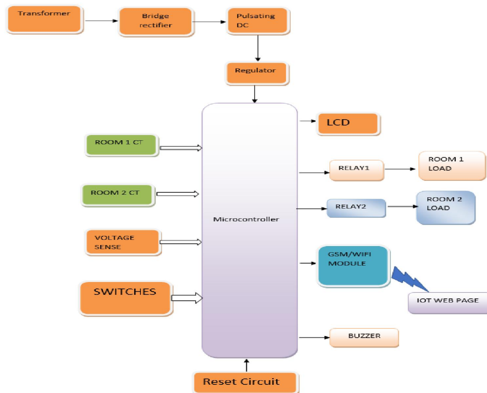
Fig.1. Block Diagram
