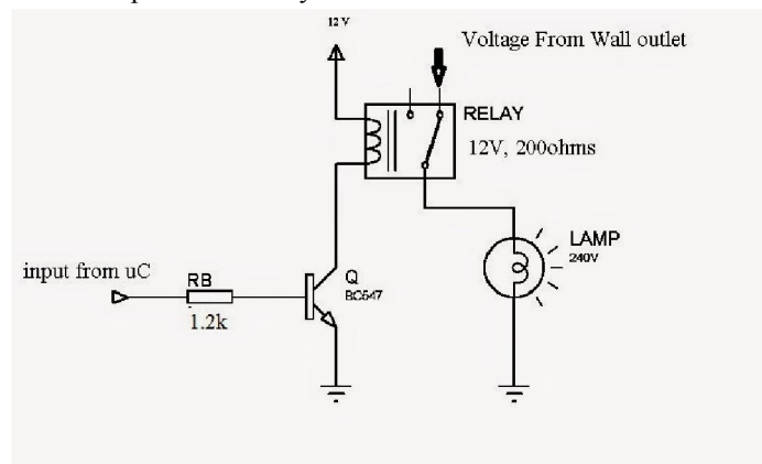
Fig. 4. Relay Driver Circuit
