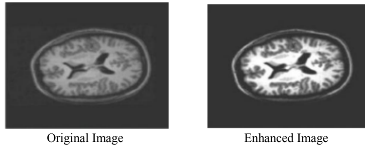
Figure 2: Image Enhancement [8]
