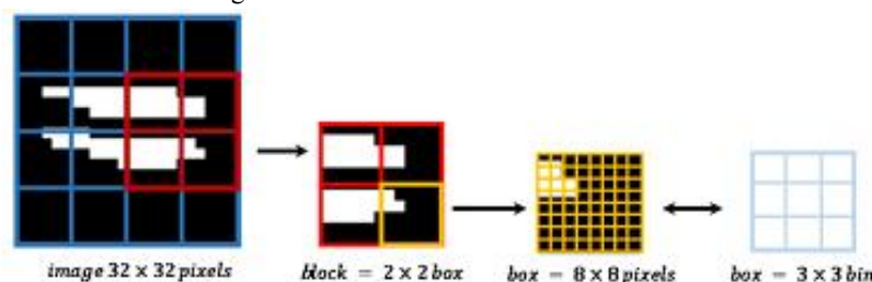
Figure 4: Architecture of HOG feature (elongated cell) [18]
