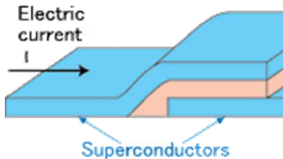
Figure 6: A thin layer of insulator is placed between two superconductors and the current reaches a certain volume where the electrons are able to pass through the insulator as if it is non-existent which can be used to switch from on to off or other way around at very high speeds. This phenomenon is called the Josephson effect. pressure than conventional superconductors. To test
