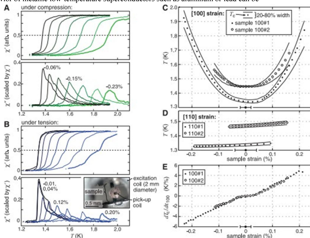
Figure 7: “Superconductivity of Sr 2 RuO 4 under strain. (A and B) In-phase (c') and out-of-phase (c'') parts of the ac susceptibility, measured at 369 Hz on the <100>-oriented sample shown in the inset of (B). Approximate strains for some curves are indicated. arb. units, arbitrary units. (C) T c versus <100>-oriented strain ε 100 of two samples of Sr 2 RuO 4 , one with a zero-strain T c of 1.35 K [for which the raw data are shown in (A) and (B)] and the other with 1.45 K. (D) T c versus <110>-oriented strain ε 110 . (E) dT c /dε 100 versus sample strain (%).
