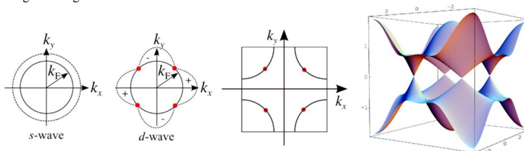
Figure 4: In the Cooper pairs of conventional superconductors, the wave functions are as symmetrical as possible: they have spherical or s-wave symmetry. That is, the probability of a paired charge carrier relative to the other falls equally exponentially of the wave function, with one of the two particles in the centre, the probabilities of finding the partner in all directions of space. In a graphical representation appear as concentric spheres. The next, slightly lower degree of symmetry is the d-state. In the diagram, it resembles four-leaved clover, with each leaf representing an area in which
