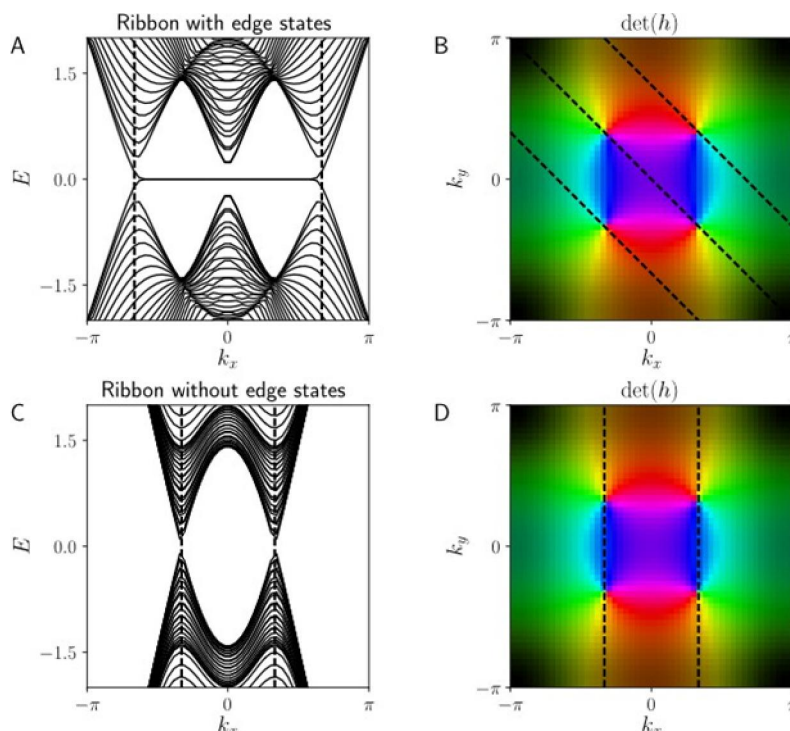
Figure 3: When the line corresponding to a constant k_{||} crosses a Dirac point, the winding number of the Hamiltonian H(k_{||}) changes by the winding of the Dirac point. Which means certain values of momentum parallel to the boundary, a zero energy edge state will occur. In a d-wave superconductor only for some crystalline orientations this will occur. On the right, \det h is seen, with lines corresponding to different values of k_{||} passing through the Dirac points. If the sample boundary happens to be along the (1,0) axis, the Dirac points will have coinciding
