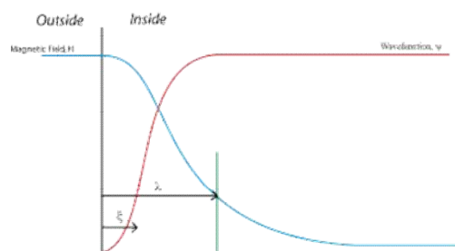
Figure 1.b: Type II Superconductors have two critical field strengths; from the lower one, the field begins to penetrate; in the higher one, the superconductivity collapses. In the area in between, the magnetic field increasingly penetrates the conductor in the form of microscopically fine tubes temperatures (around 300 K), this would most likely profoundly change modern technology.
