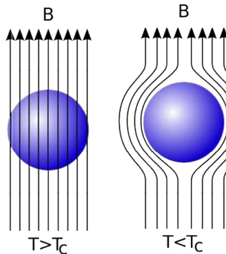
Figure 5: When a superconductor is put under magnetic field, some electric current passes through it to cancel out the field which keeps the magnetic field outside. This is called the Meissner effect.
