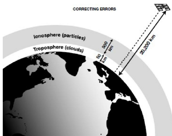
Fig. 8: Atmospheric Effects in the Troposphere and Ionosphere [2]
