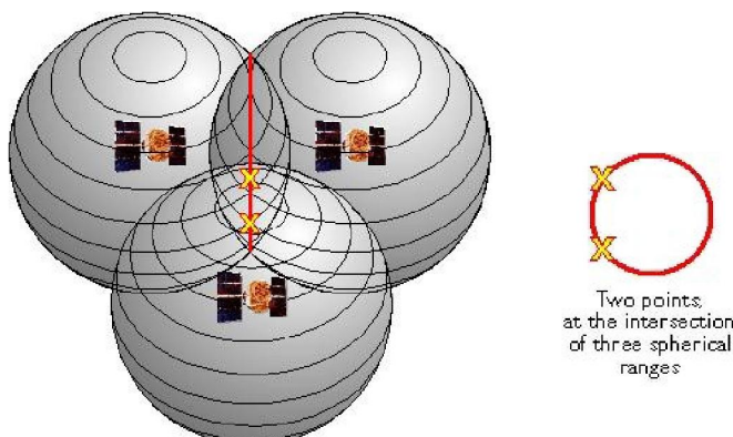
Fig. 4: Third measurement from another satellite puts the receiver at one of two points where all three spheres intersects [8]
