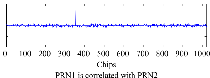
Fig. 6:(a) Erroneous GPS Satellite (Upper), (b) True GPS Satellite Match ((Lower) -PRN1 is shifted 350 bits) [11]
