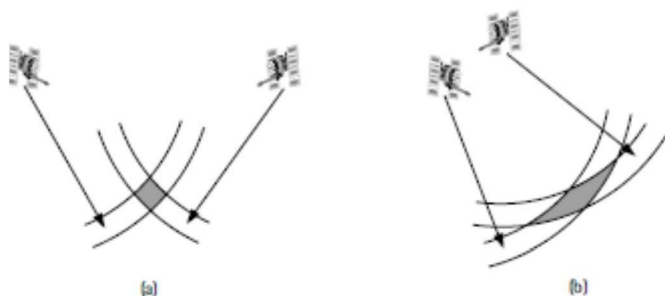
Fig. 7: (a) Good Satellite Geometry; and (b) Bad Satellite Geometry [4]
